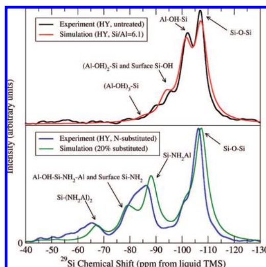
Figure 1. ^{29}\text{Si} NMR spectra of HY zeolite (Si/Al = 6.1) with 0% (top), 20% of oxygen substituted for NH groups.
